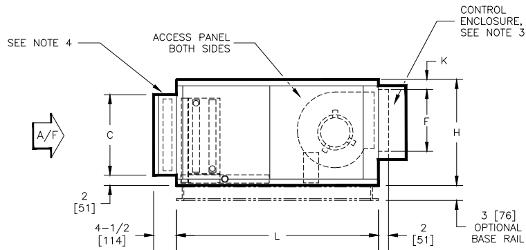
STANDARD FILTER RACK
