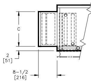
HIGH EFFICIENCY FILTER RACK
