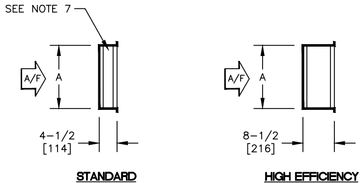
SIDE VIEWS
